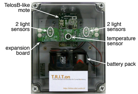
Figure 4: A deployment-ready WSN node.
