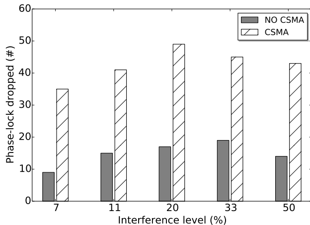
Figure 6. Number of phase-lock losses when using default ContikiMAC with and without CSMA.
