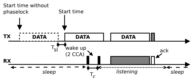
Figure 2. After the neighbour schedule is learned, the phase-lock mechanism reduces the length of the transmission.
