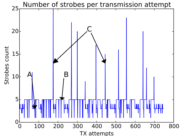
Figure 4. Number of strobes used for each transmission attempt with the original design of ContikiMAC and an interference level of 20%.
