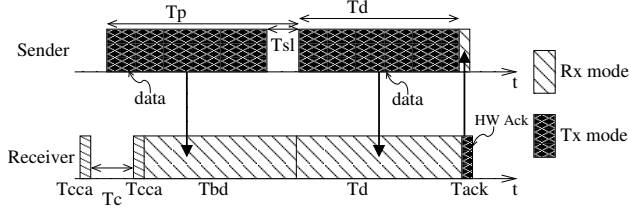
Figure 3. Unicast transmission in ContikiMAC.
