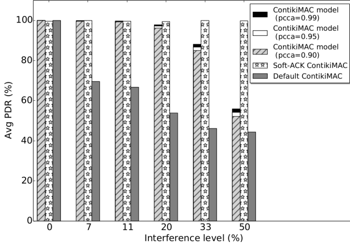
Figure 8. PDR results with CSMA. Soft-ACK ContikiMAC increases performance and our model establishes a lower bound even under high interference.
