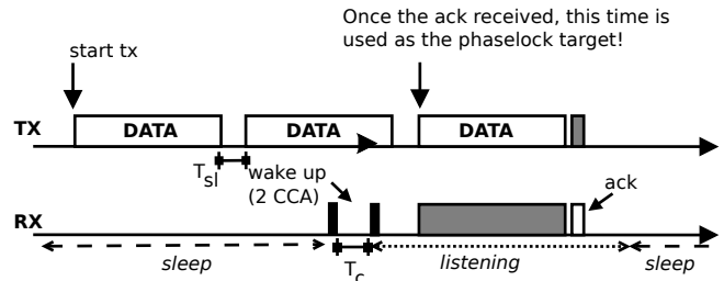
Figure 1. When an ACK is received, the sender can estimate the wake-up schedule of the receiver.
