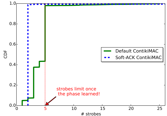
Figure 5. Number of strobos sent by transmission attempt with interference during 20% of time. Soft-ACK ContikiMAC mostly uses only two attempts demonstrating its effectiveness.
