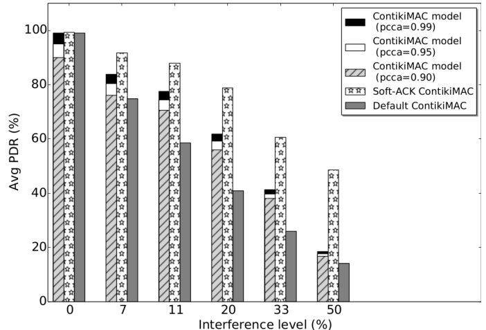
Figure 7. PDR results without CSMA. Soft-ACK ContikiMAC increases performance by avoiding loss of phase-lock. Our model establishes a lower bound.
