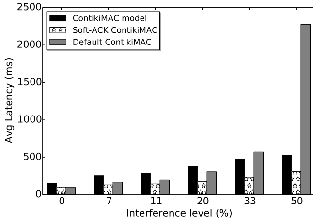
Figure 9. Latency results with CSMA. Avoiding loss of phase-lock has a huge impact on latency. Our model provides an upper bound (worst case) for soft-ACK ContikiMAC.
