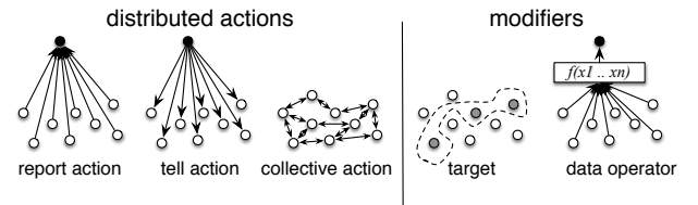
Figure 3. Distributed actions and modifiers.
