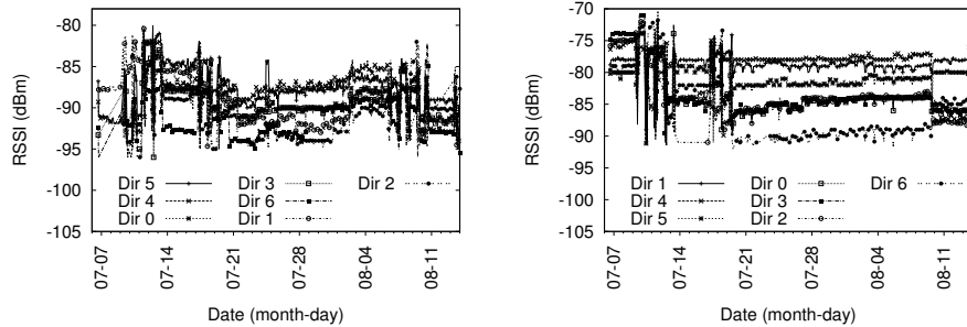
(a) Node 6: non-LOS conditions, TX power 17, channel 19. (b) Node 2: non-LOS conditions, TX power 5, channel 15.
