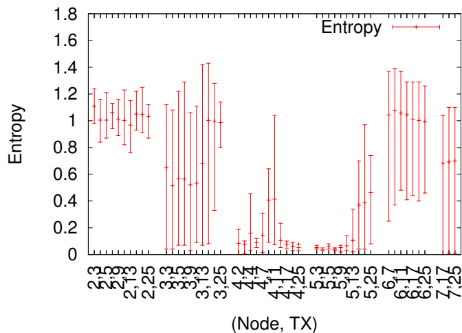
Fig. 5: Average, maximum, and minimum entropy of best performing antenna direction depending on receiver node and TX power.
